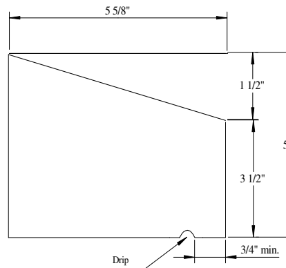
Section S-4
