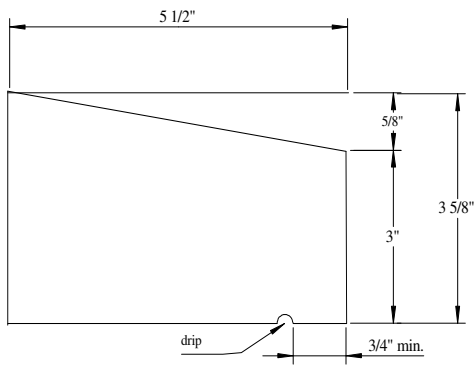
Section S-1
